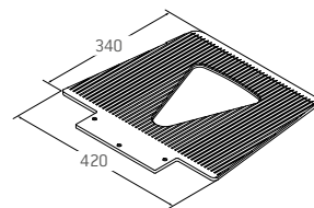
Toe plate G (420x340x7 mm) for large loads Art. no. 930 003
