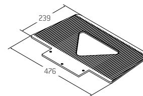
Toe plate GS (476x239x7 mm) used in the beverage industry for barrels and crates Art. no. 930 030
