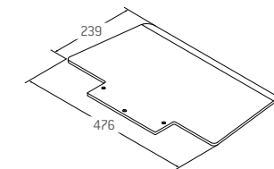
Toe plate GS-NG (476x239x7 mm) for goods in cartons (e.g. beverage cans) Art. no. 930 084
