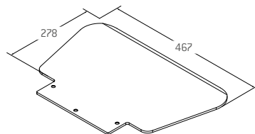
Toe plate LH (467x278x5 mm) like toe plate V, but larger Art. no. 930 002
