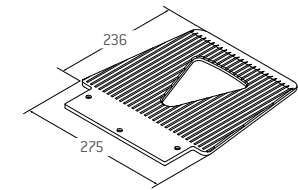
Toe plate Standard (275x236x7 mm) with grooves to prevent load slipping sideways Art. no. 030 025
