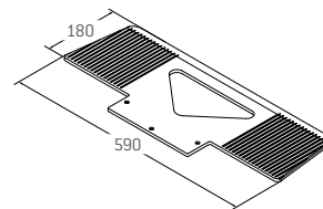
Toe plate XWL (590x180x7 mm) also for white goods, feet stand on toe plate Art. no. 930 074
