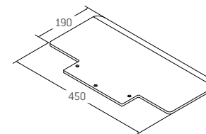
Toe plate DS-NG (450x190x7 mm) also for carton-packed goods Art. no. 930 085
