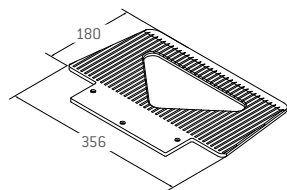
Toe plate WL (356x180x7 mm) suitable for white goods, refilling vending machines, etc. Art. no. 930 018
